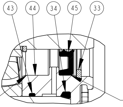
SINGLE SHAFT SEAL ASSEMBLY P2-075-0210-01□ SECTION A-A SCALE 1:1
